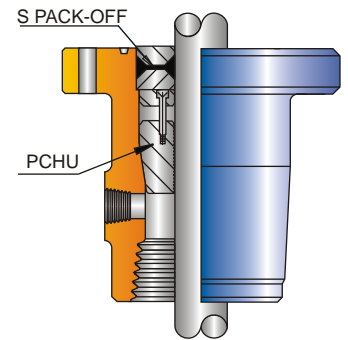
Type 'PCHU' Unitised Casing Hanger with Slip Seal Assly
