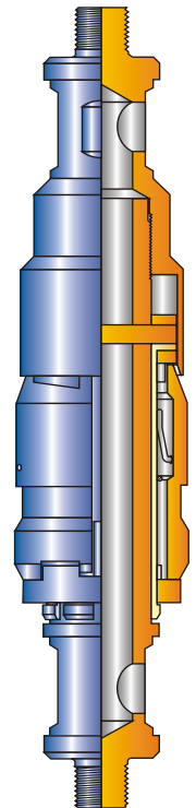
B SHIFTING TOOL
