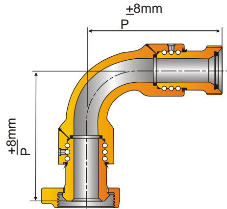
STYLE - 60 LONG SWEEP SWIVEL JOINT END CONNECTION = UNION (M X F) FIG.602/1002/1502* MODEL:- PLSSJ - 60MF
