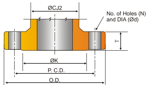
Integral Flange
