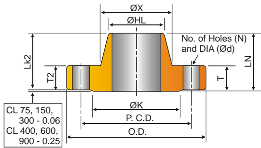
Weld Neck Flange
