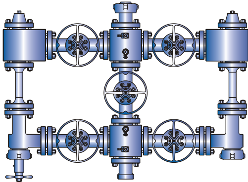
Choke Manifold
