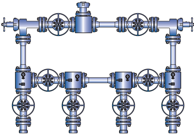
Eruption Manifold
