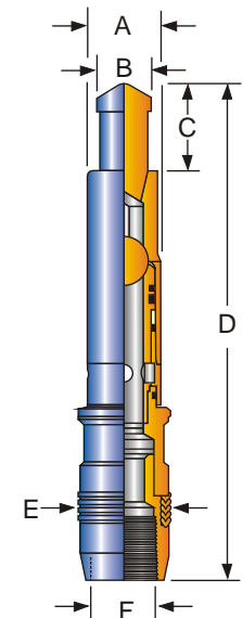
TYPE E-3 STANDING VALVE
